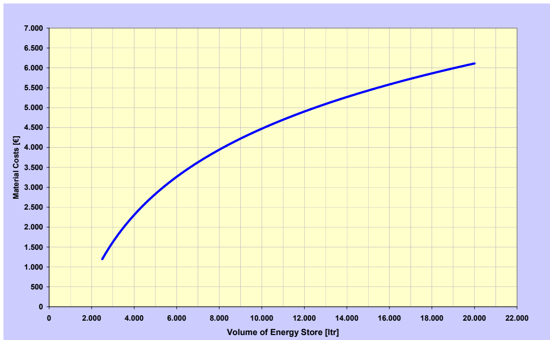
Figure 112: Progression of the costs of the energy storage tank depending on the volume based on results from cost proposals from realised projects (exclusive taxes).
