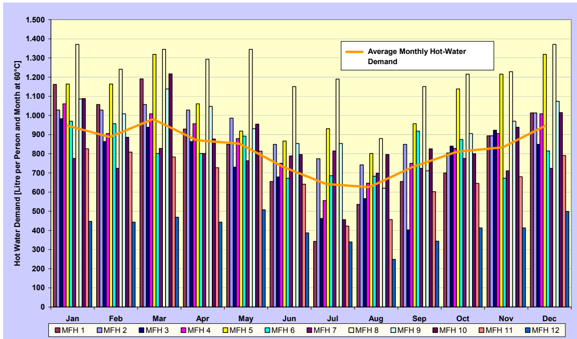
Figure 15: Measured monthly domestic hot water consumption from 12 multi-storey residential buildings during one year. The mean daily domestic hot water demand is just under 30 litres per person and day at 60 °C (Fink et al., 2002; Luboschnik et al., 1997, Gassel, 1997).
