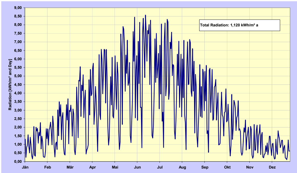
Figure 12: Solar radiation on a horizontal area in Graz, Austria, created from mean month temperatures generated from values over many years.
