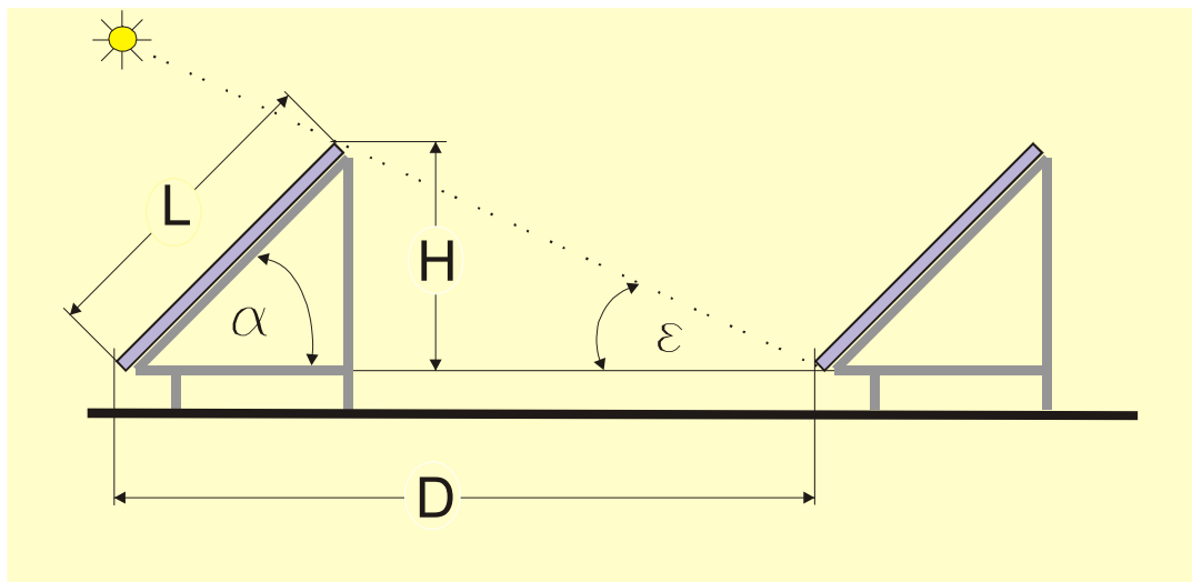
Figure 33: Variables influencing the distance, D between the assembly rows.
