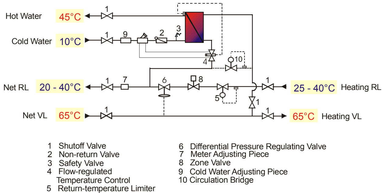
Figure 71: Block diagram of the functional layout of the components in an apartment unit and allocation of the typical operating temperatures.
