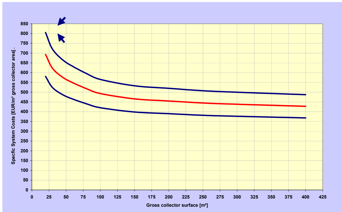
Figure 110: Progression of the specific solar thermal system over the gross collector area: the red line shows the mean system price, the two blue lines show the possible effect from the specific basic conditions of the project. The specific prices do not include taxes, planning costs or subsidies.
