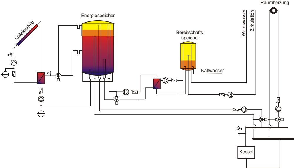
Figure 87: Concept for a two-tank system for solar-supported heating of domestic hot water for more than 10 apartments.
