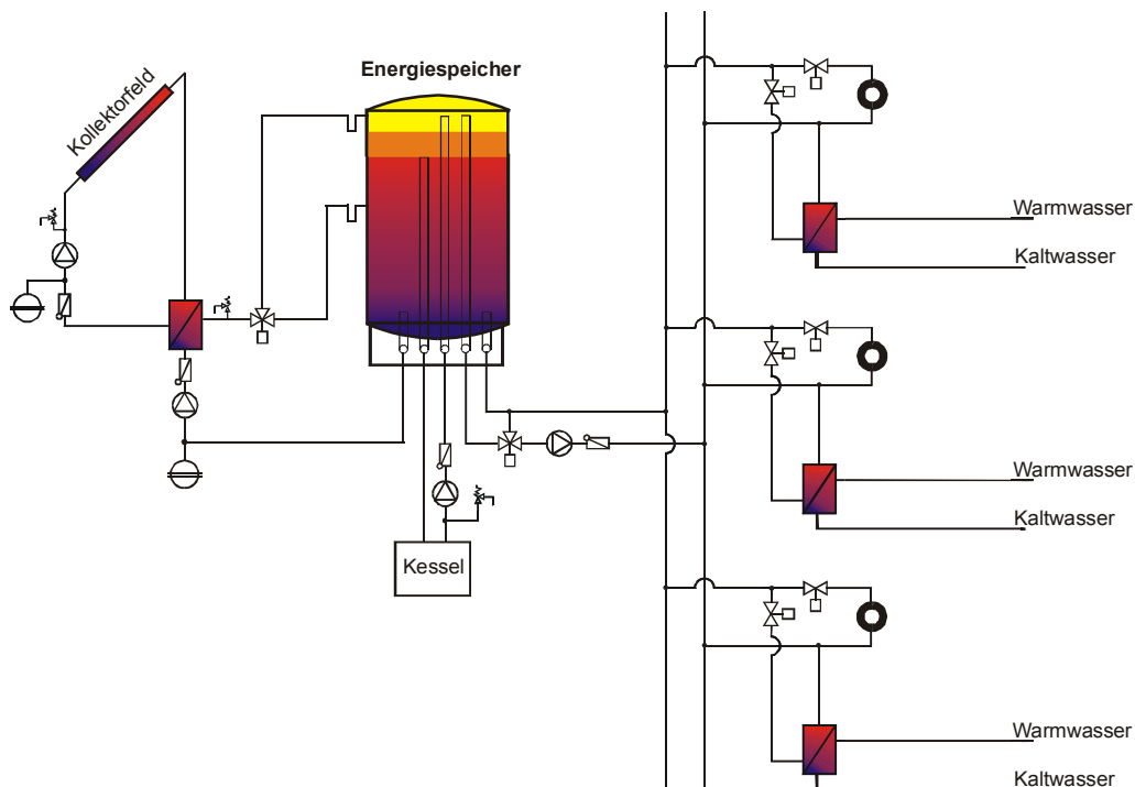
Figure 81: Solar-supported concept for heat distribution: two-pipe networks connected with the decentralised domestic hot water storage tank.
