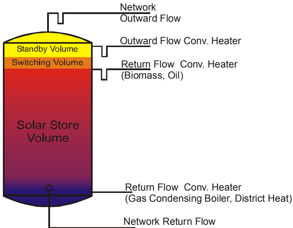
Figure 97: Block diagram showing the storage management in solar-supported heat supply concepts with the two-pipe network principle.
