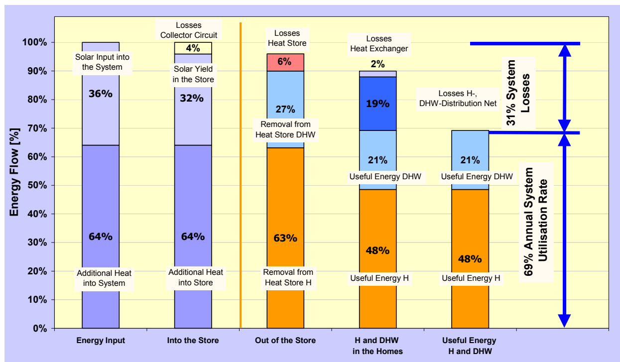
Figure 7: Exemplary description of the system losses of a solar-supported heating supply system (from the heat distributor to the end user with an annual degree of system utilisation of 69%).
