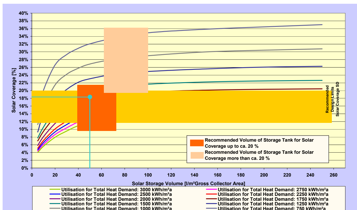
Figure 92: Nomogram to determine the gross collector area and the volume of the storage tank in relation to the solar coverage. The dark yellow area shows the recommended design limits in the cost-benefit optimisation. The sensible areas to determine the specific volume of the storage tank depend on the solar coverage and are shown as rectangles. The green lines are help lines for a dimensioning example.
