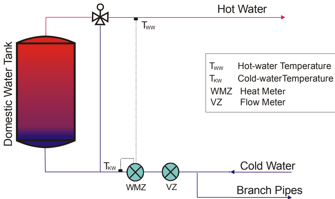
Figure 16: Correct functional assembly of volume flow and temperature measuring devices (volume part and temperature sensors).
