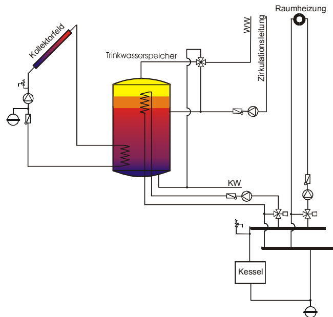
Figure 85: Solar-supported heating of domestic hot water for a maximum of 10 apartments using single tank storage systems. The hot water is stored in a domestic hot water storage tank.
