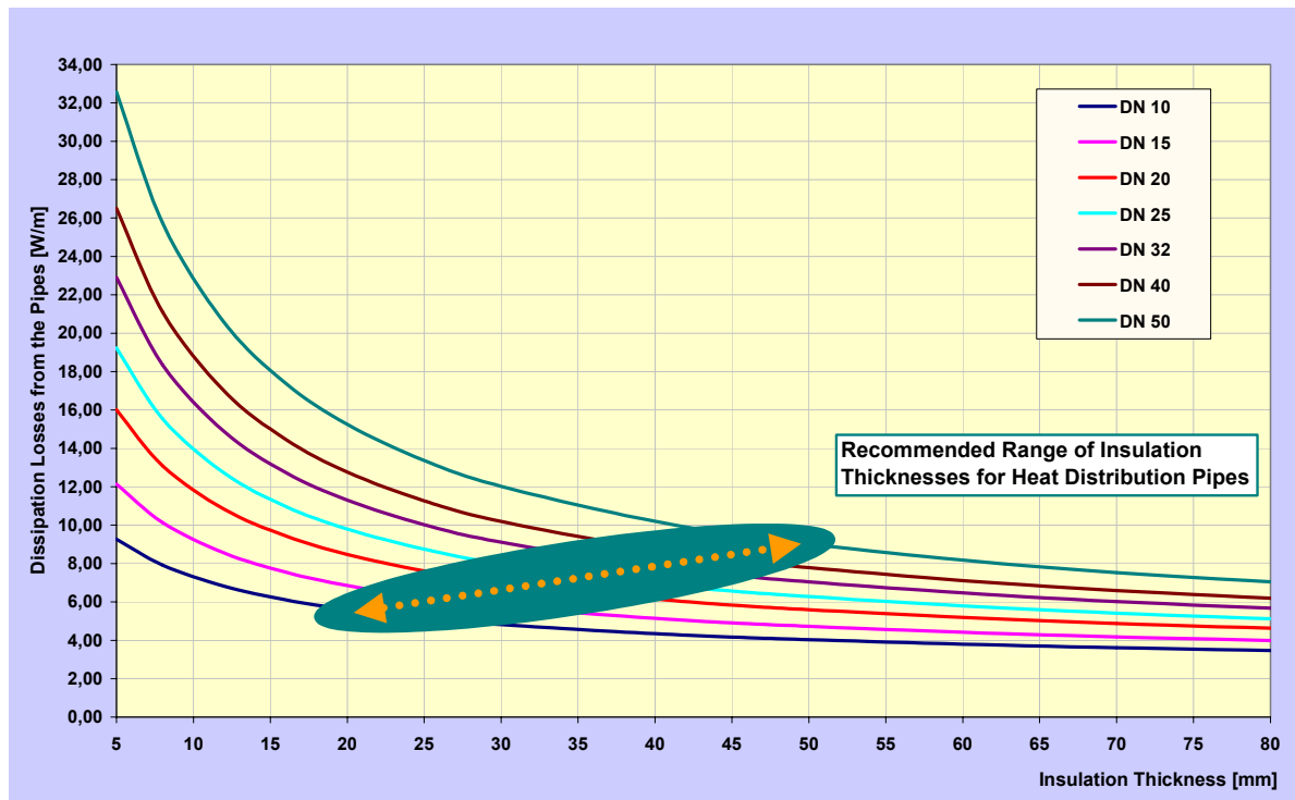
Figure 104: Theoretical dissipation losses (Watt per meter of pipe) depending on the pipe dimension and the insulation thickness (the graphic is based on: \lambda_{insulation} = 0,04 \text{ W/mK} , \epsilon_{coat} = 0,5 and a temperature deviation of 40 K between the medium and the surroundings).
