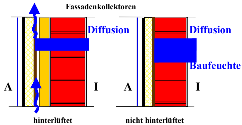
Figure 36: Moist diffusion in wall constructions with back-ventilated and not back-ventilated façade collectors.
