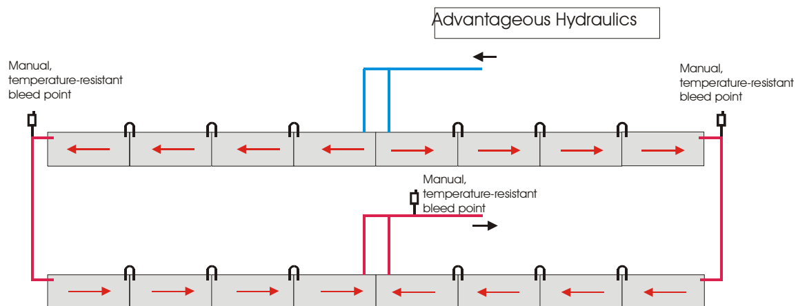
Figure 54: Example of collector interconnection for flat roof installations with 160 m 2 gross collector area: there is hardly need for pipe works because of the serial connection by big size collector area.
