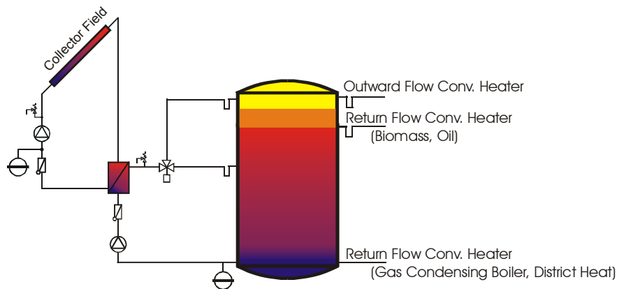
Figure 63: Charging of the storage tank at one level – just below the standby volume.
