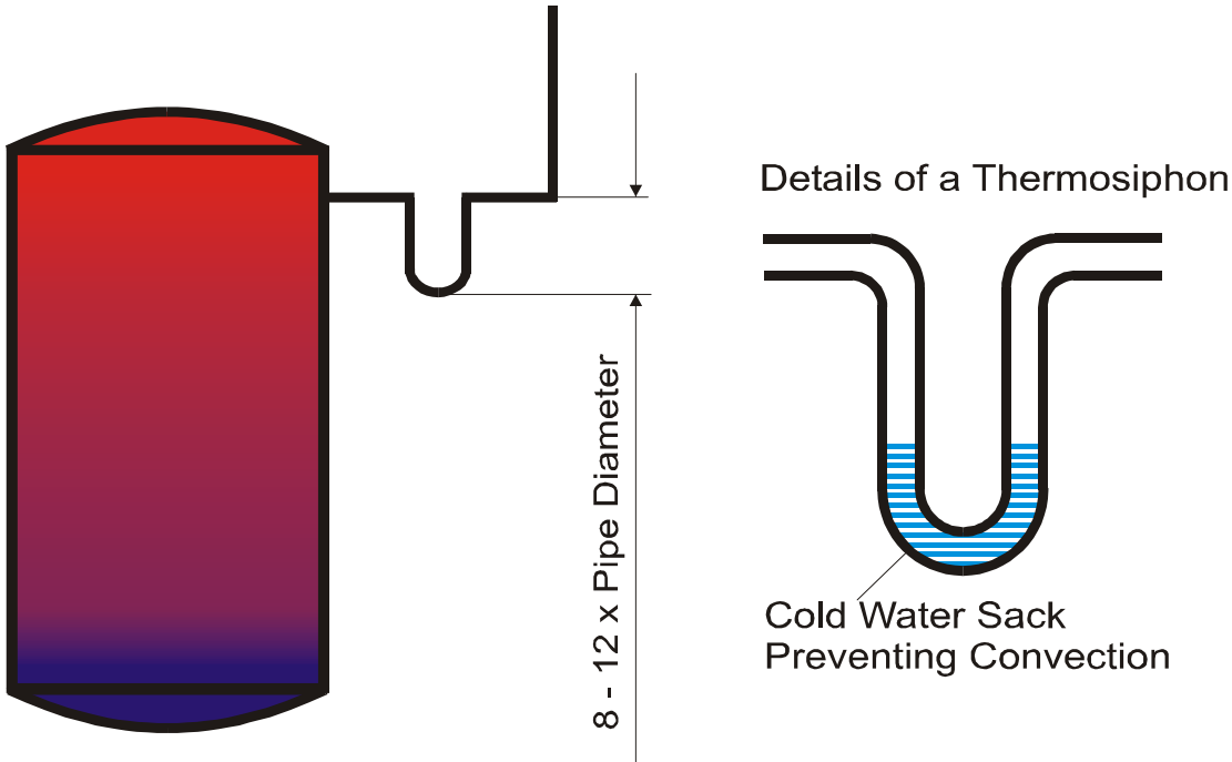
Figure 99: A thermosiphon with a depth of at least 8 times the diameter of the pipe prevents internal circulation in the pipe.
