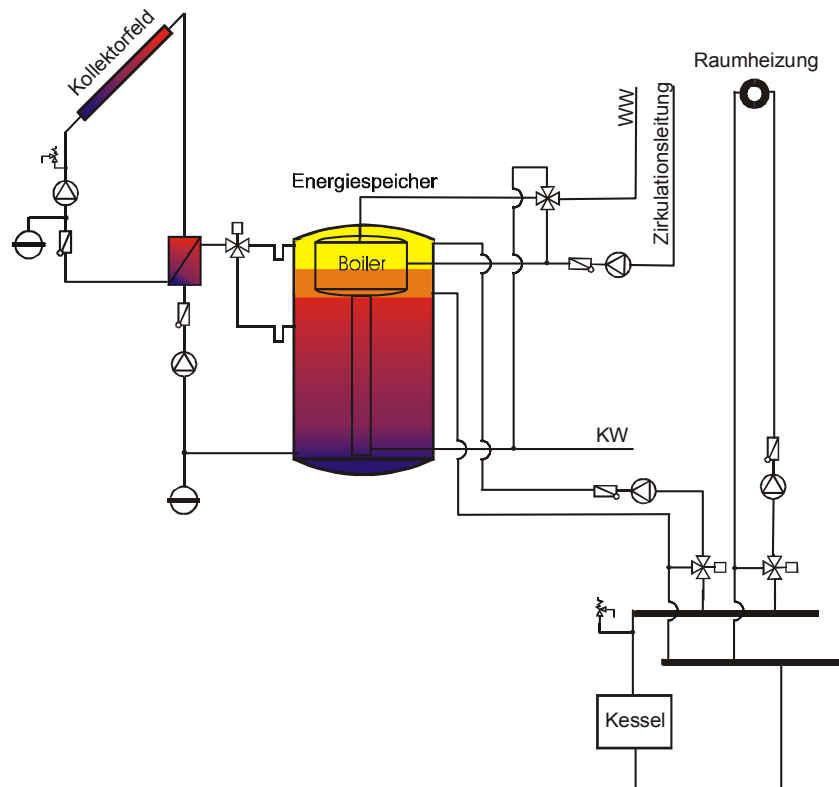
Figure 86: Solar-supported heating of domestic hot water for a maximum of 10 apartments using single tank storage systems. The hot water is stored in a conventional uncoated steel tank connected with an integrated domestic hot water tank.
