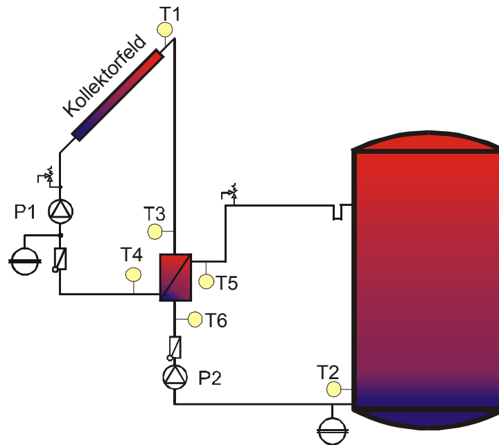
Figure 49: Allocation of the temperature sensors corresponding to the speed control criteria of the primary and secondary pump, listed in table 4.
