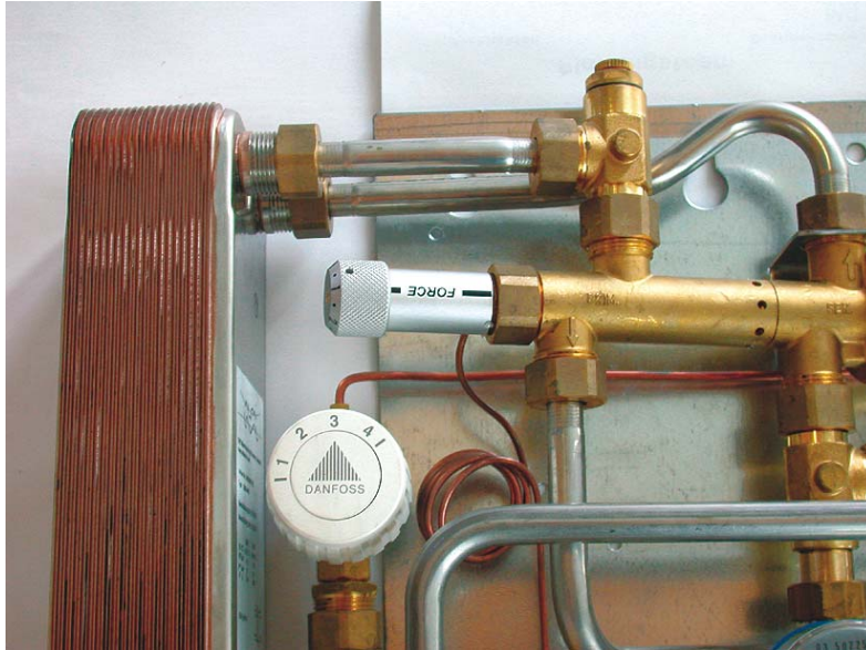
Figure 72: Components for heating the domestic hot water – plate heat exchanger, adjustable proportional controller and circulation bridge with return temperature limiter (example from the product from the Redan company) (picture source: AEE INTEC).
