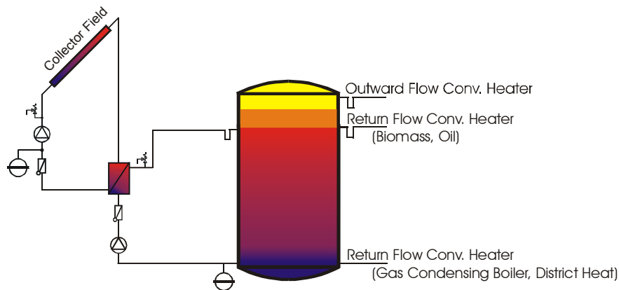
Figure 62: Temperature oriented charging in two levels of the storage tank.
