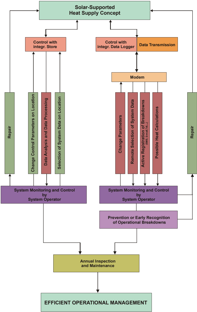
Figure 115: Illustration of the different regulation and monitoring possibilities for solar-supported heat supply concepts for multi-storey residential buildings.
