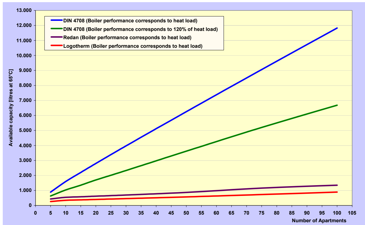
Figure 96: Necessary available volume capacity depending on the number of apartment units. Comparing the DIN 4708 (blue and green line) with the dimensioning recommendations. This diagram is based on: 3 kW heat demand per apartment, 36 kW maximum domestic hot water demand per apartment, 40 K as \Delta T for the hot water preparation, 25 K as \Delta T for the heating boiler circulation.
