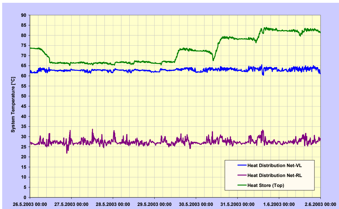
Figure 80: The satisfying mixer function of thermal tank at high storage temperatures can clearly be recognised (end of May/beginning of June). The supply temperatures are constant and just below 65°C, the return temperatures lie between 23 and 33°C.
