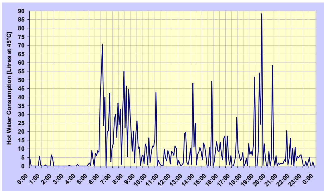
Figure 18: Daily consumption profile for multi-storey residential buildings, constructed through measurements and probability calculations for an example with a daily domestic hot water consumption of 2000 litres at 45 °C (Weiß, 2003).
