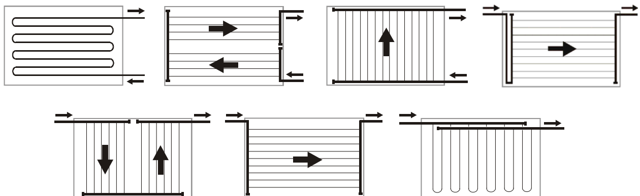
Figure 59: Evaluation of different outflow behaviour in the stagnation condition.
