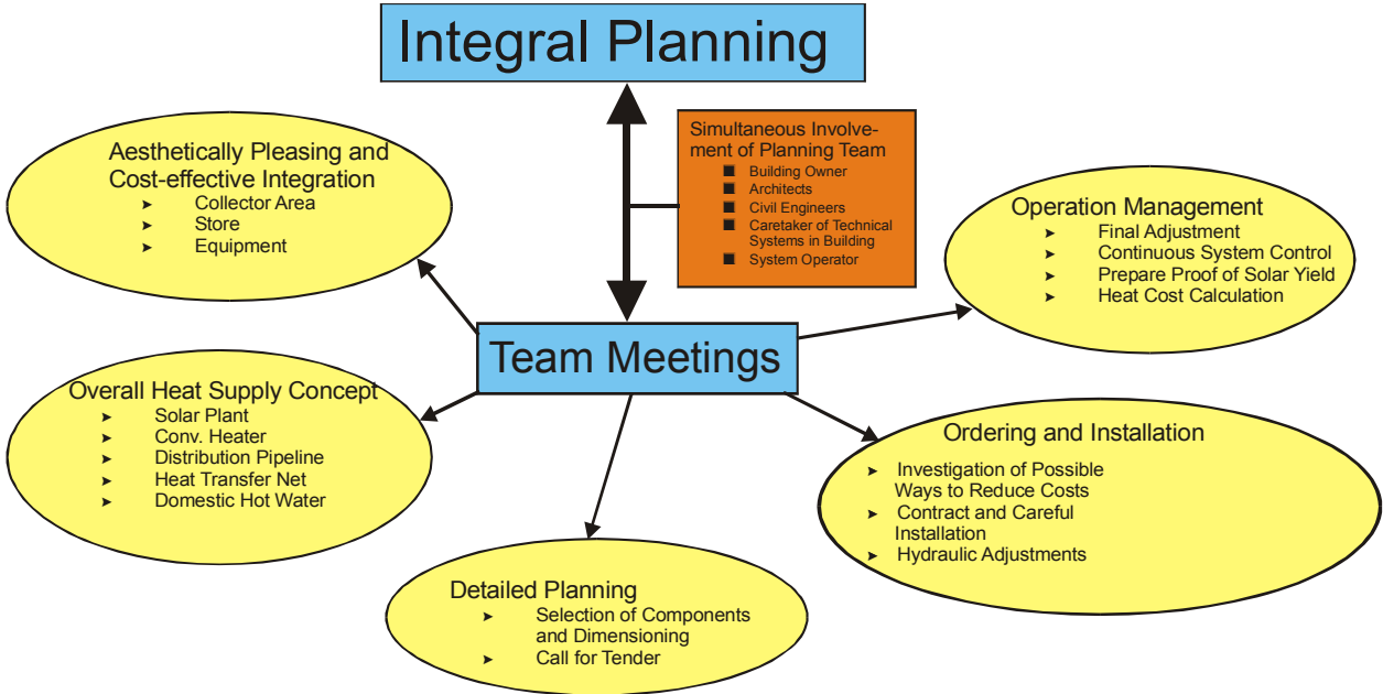
Figure 5: Method for the holistic use of applied solar-supported heating systems.
