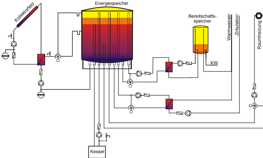
Figure 88: Concept for a two-tank system for solar-supported heating of domestic hot water and space heating for more than 10 apartments. Further is the return water reheated through an internal heat exchanger over the circulation line.
