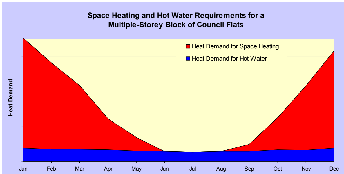
Figure 14: Space heating and domestic hot water requirements for a multiple-storey block of council flats (25 flats, heating load: 100 kW, 80 m 2 collector area, solar coverage: 18%).
