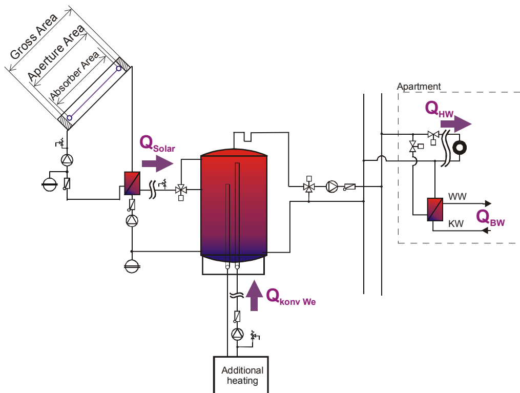
Figure 47: Allocation of the heat flow and reference values in the solar thermal system.
