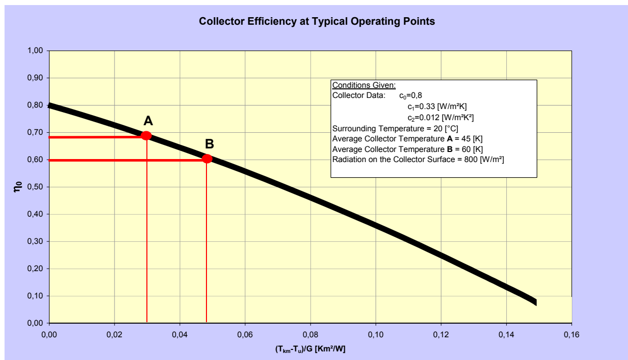
Figure 6: The influence of the temperature on the achievable collector efficiency. An Adapted holistic heating systems with lower mean temperature (operating point A) achieve essentially higher collector efficiency than for the example a solar thermal system with high return temperatures in the heat distribution system (operating point B).
