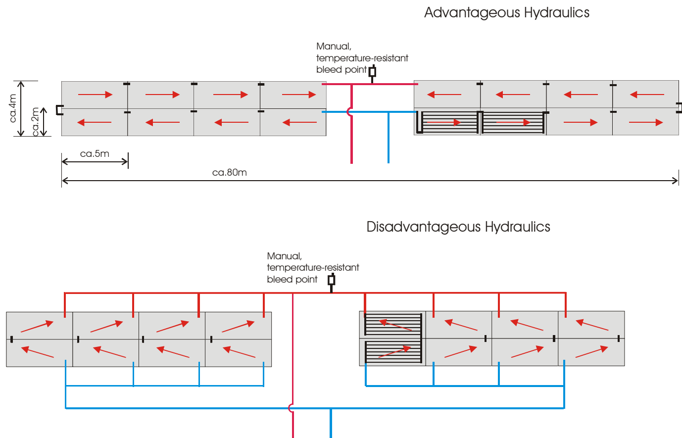
Figure 52: Two examples of collector interconnections for a roof integrated collector area with 160 m 2 gross area: there is hardly any need for pipe work in the upper hydraulic. The lower hydraulic need an additional 90 m pipe work.
