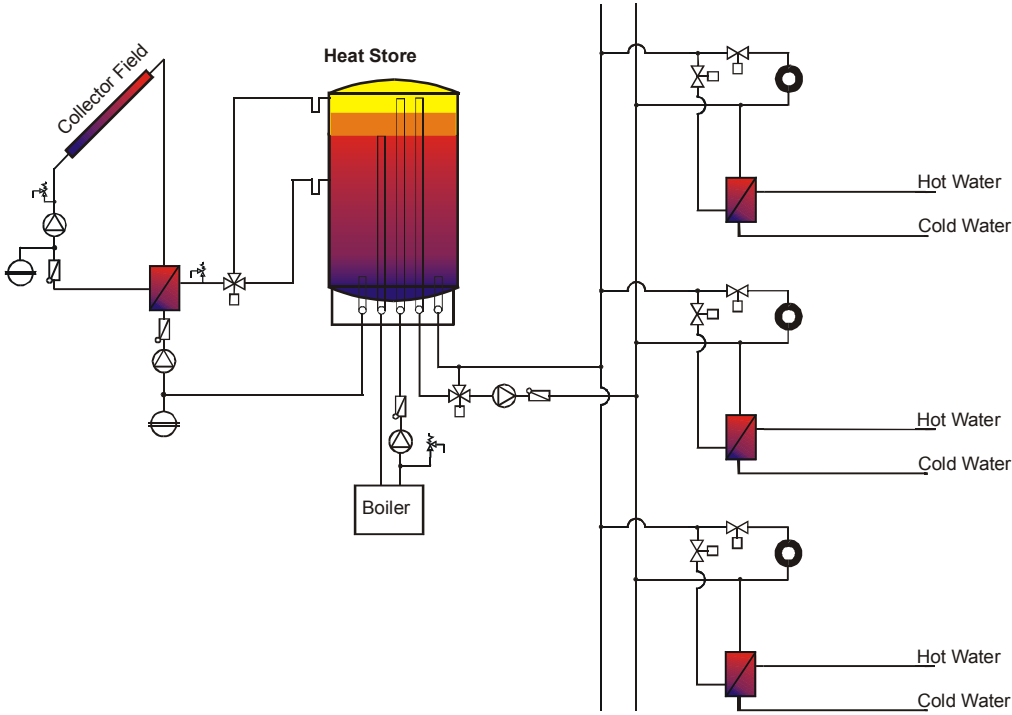
Figure 65: Solar-supported heat supply concepts: two-pipe network connected to the decentralised apartment unit.
