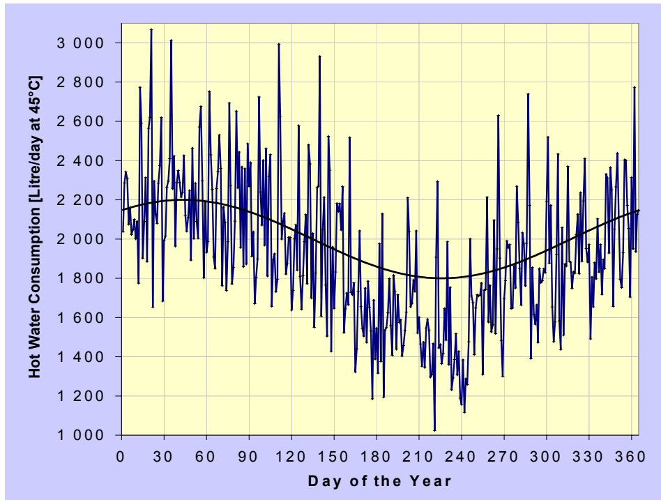
Figure 19: Annual consumption profile generated from the daily consumptions profile where measurements and probability calculations (with a daily mean domestic hot water consumption of 2000 litres at 45 °C) are taken into account (Weiß, 2003).
