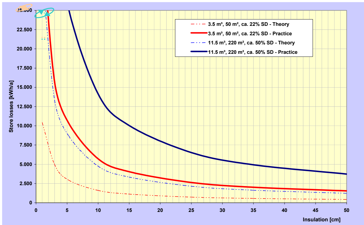
Figure 98: Isolation material depending on the solar coverage – differences between theory and practice. An insulation material with the heat conductivity of 0,042 W/mK was used (Heimrath, 2004).
