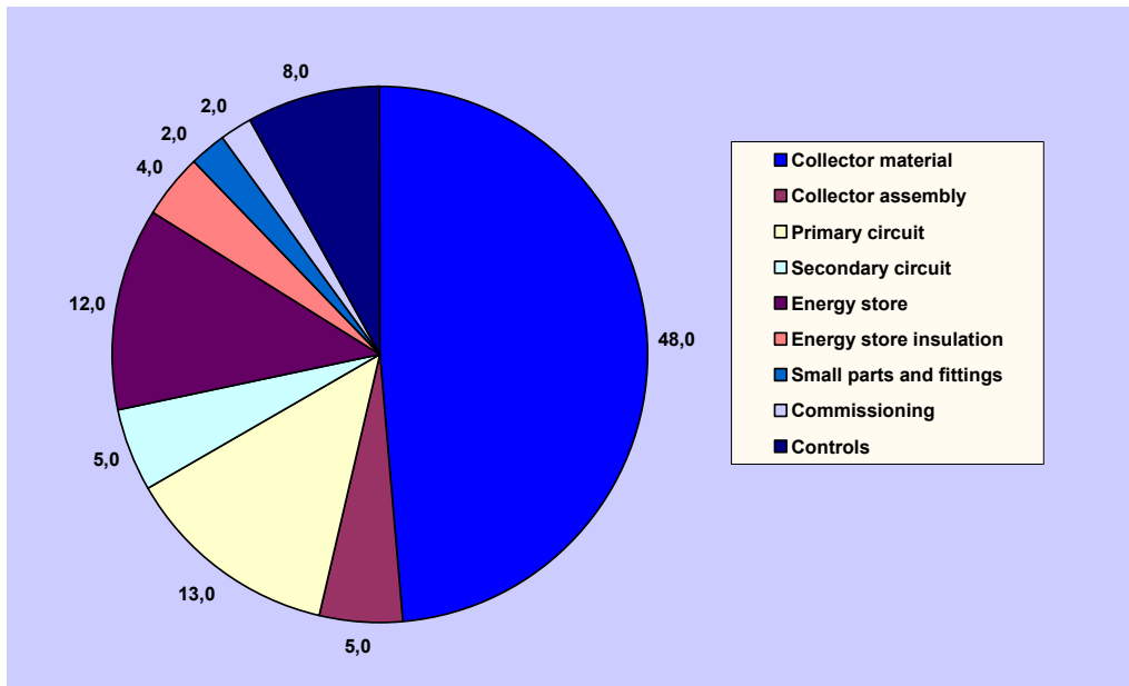
Figure 111: Average solar system costs divided in costs groups based on results from cost proposals from realised projects (exclusive taxes).
