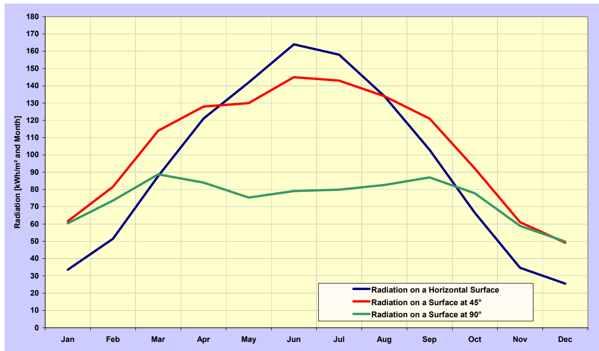
Figure 13: Average annual global irradiation in three areas at a different incline, Graz, Austria.
