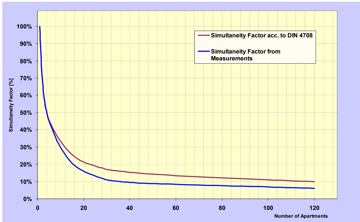
Figure 95: Simultaneity Factor according to DIN 4708 and measurements (source: Recknagel et al., 2003).
