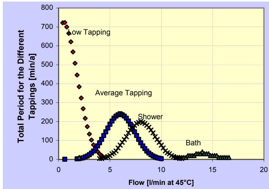
Figure 17: Progression of withdrawal time during different tapping categories as a function of the tapping flow (Weiß, 2003).
