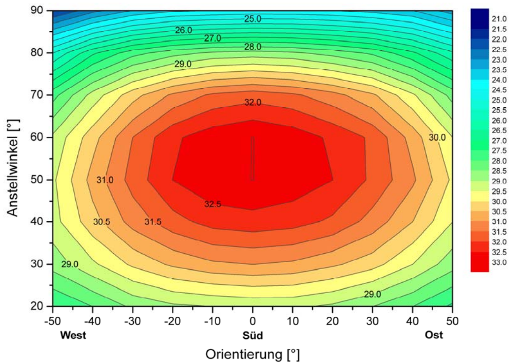
Figure 93: Nomogram to determine the reduction of the solar coverage in relation to the actual inclination and the actual orientation (valid for solar coverage around 30%).
