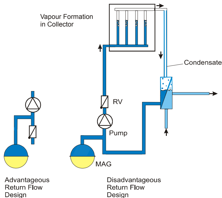
Figure 60: The stagnation behaviour depends on the return valve design.
