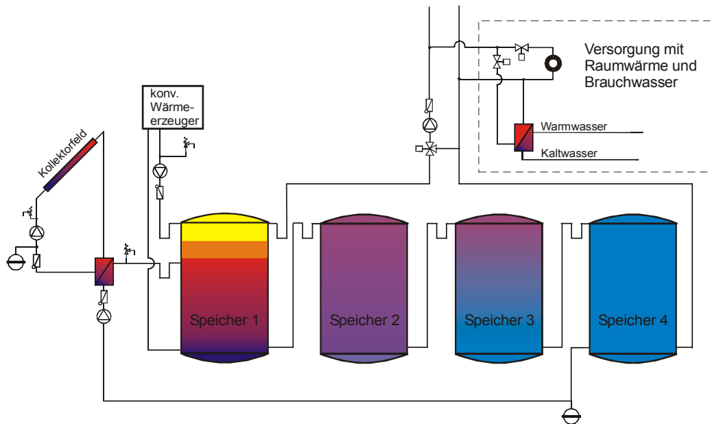
Figure 103: Should a multi-storage-unit system be inevitable (for example in an existing building), is a serial connection between the single tanks recommended.
