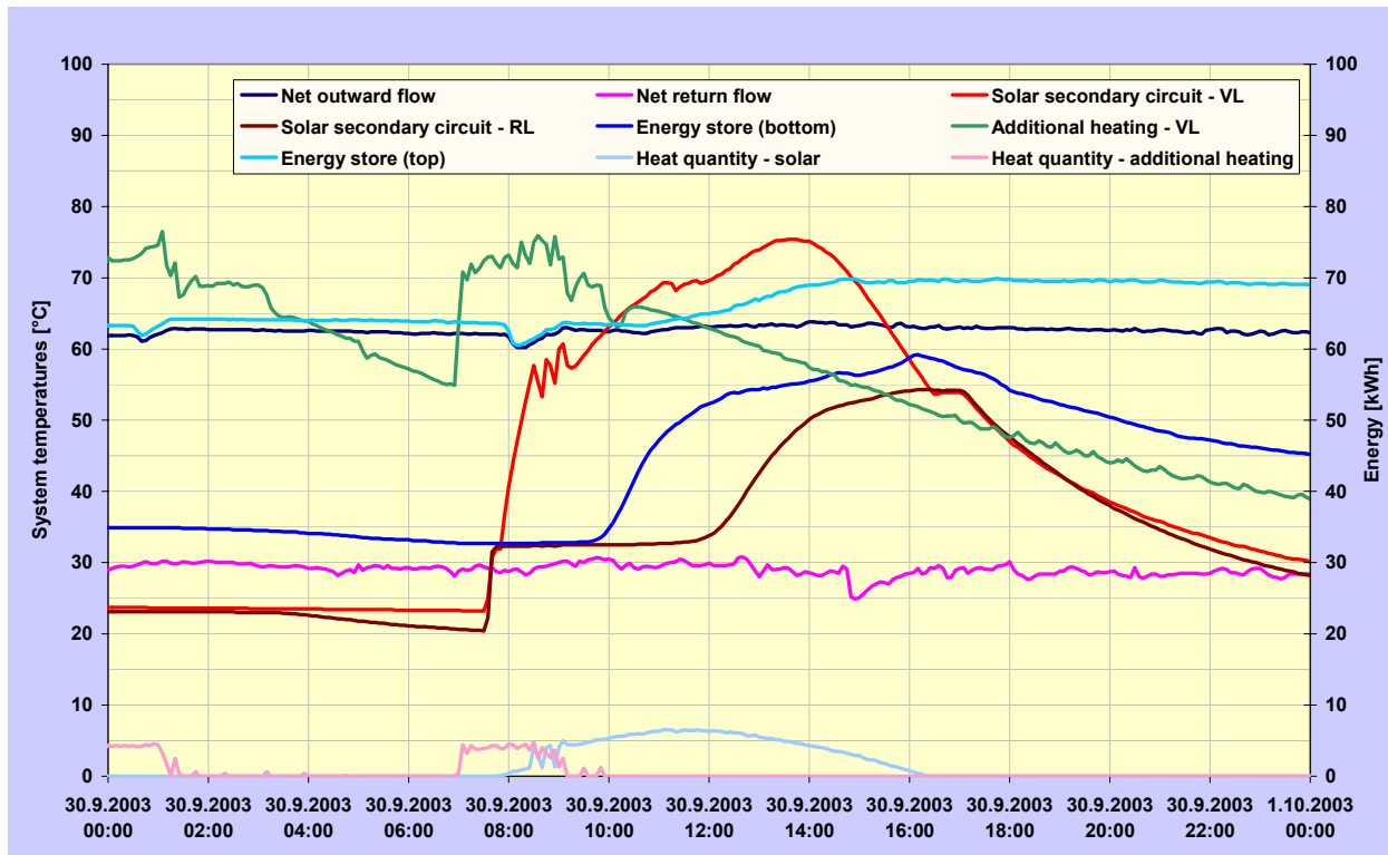
Figure 113: Important adjustments for each heating system based on temperature patterns, operation time and heat meter.
